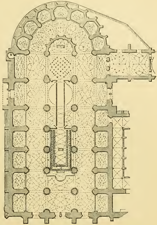
955. Plan of Cathedral at Segovia. (Reduced from Street.) Scale 100 ft. to 1 in.
