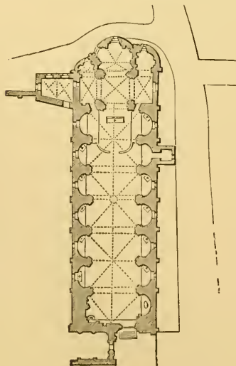
584. St. Trinité, Angers. (From Fau'trier.) Scale 100 ft. to 1 in.
