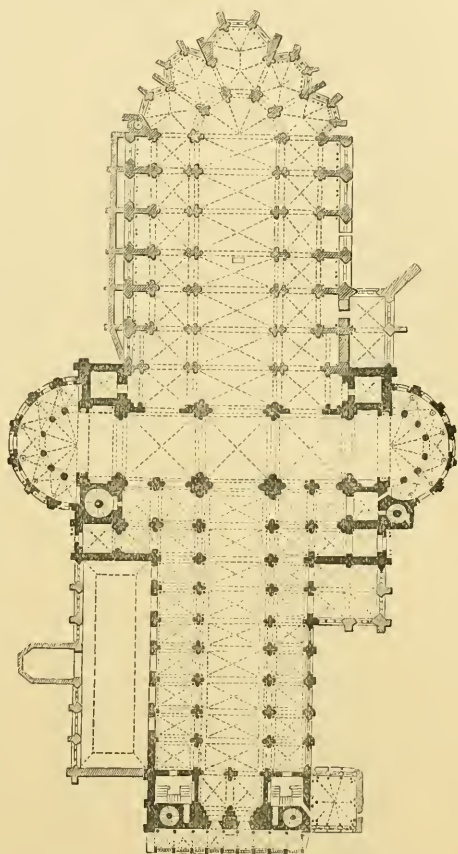
675. Plan of Cathedral at Tournay. Scale 100 ft. to 1 in.
