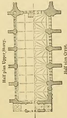
845. Plan of St. Stephen's, Westminster. Scale 50 ft. to 1 in.
