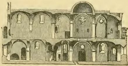
718. Section of Church of Schwartz Rheindorf. Scale 50 ft. to 1 in.
