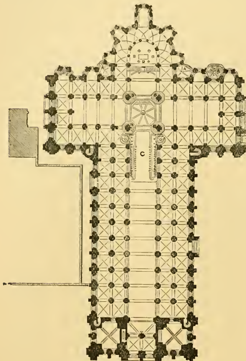
572. Church of St. Sernin, Toulouse. (From the 'Archives des Monuments Historiques.')
