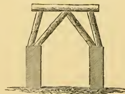
1026. Diagram of Mexican construction.
