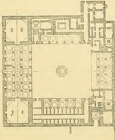
983. Plan of Mosque and Tombs of Sultan Berkook. (From Coste.) Scale 100 ft. to 1 in.
