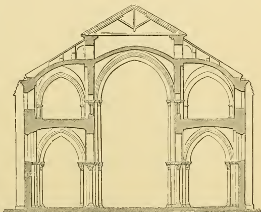
604. Section of Narthex at Vezelay. (From Didron's 'Annales Archéologiques.')
