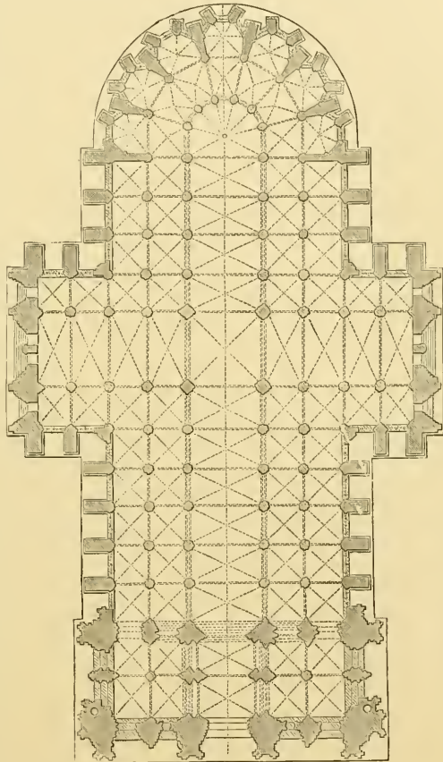
746. Plan of Cathedral at Cologne. (From Boisseree.) Scale 100 French ft. to 1 in.
