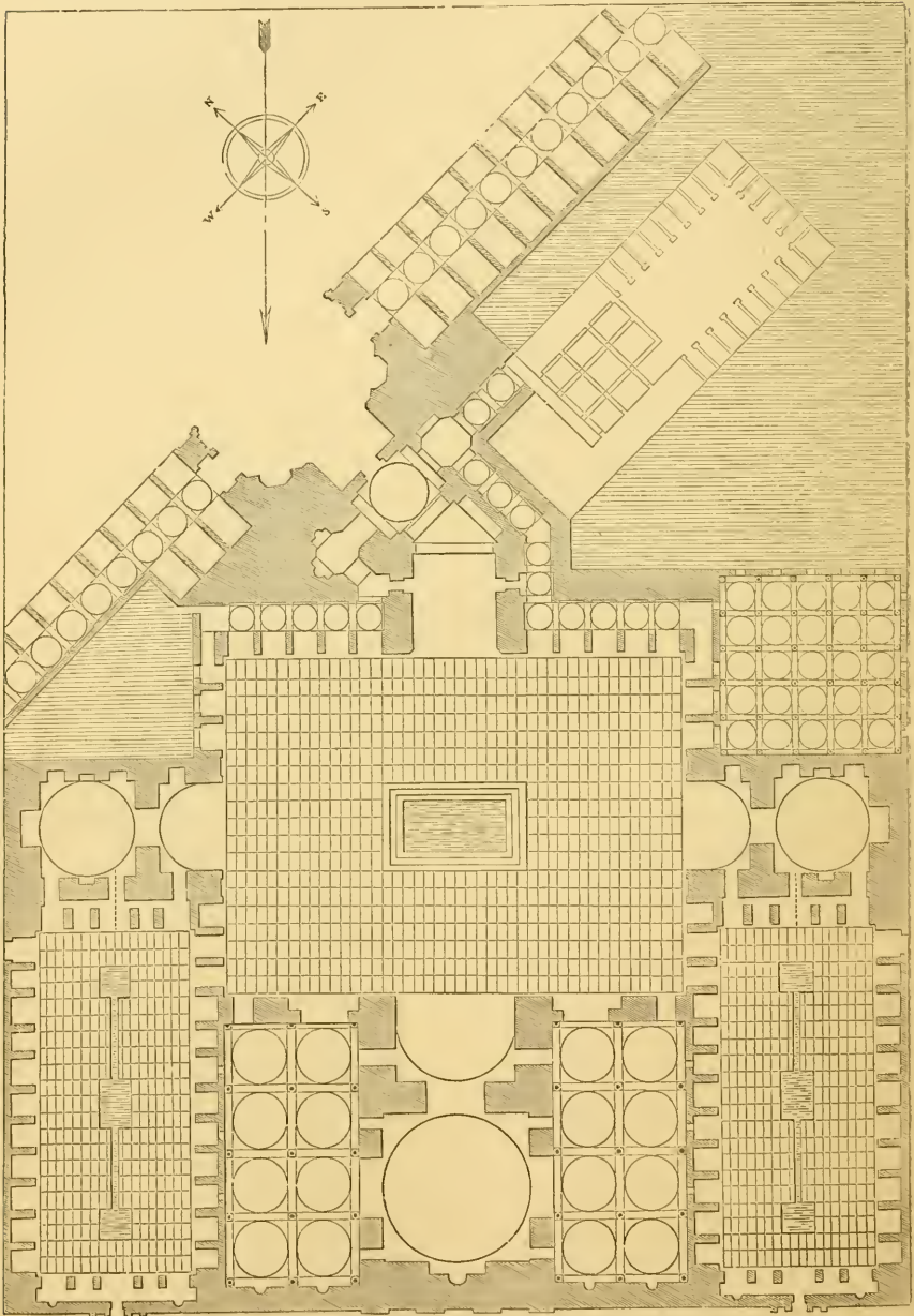
1010. Great Mosque at Ispahan. (From Texier's Work.) Scale 100 ft. to 1 in.
