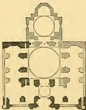
1005. Mosque at Tabreez. Scale 100 ft. to 1 in.
