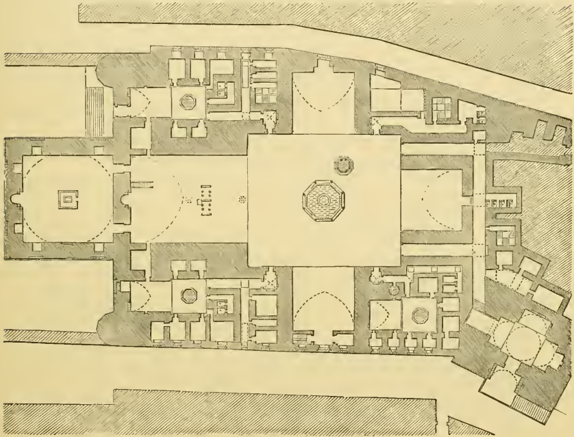
981. Mosque of Sultan Hassan. (From Coste's 'Architecture Arabe.') Scale 100 ft. to 1 in.
