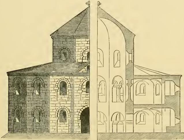
725. Church at Nymwegen. (From Schayes.) No scale.
