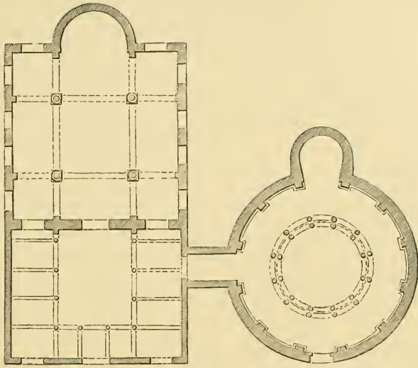
695. Plan of Original Church at Trèves. 1 Scale 100 ft. to 1 in.
