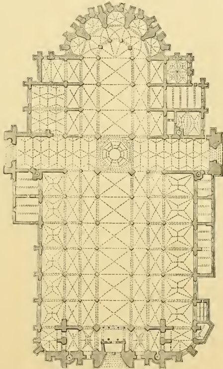
Plan of the Cathedral at Antwerp. Scale 100 ft. to 1 in.
