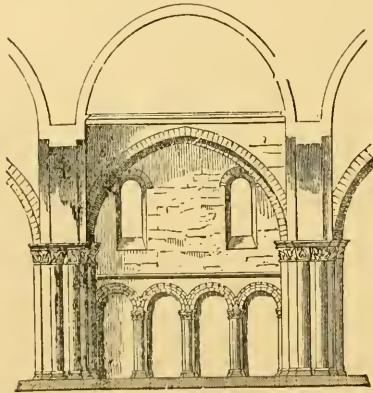
588. Elevation of one of the Bays of the Nave at Fontevault. (From Verneilh.)
