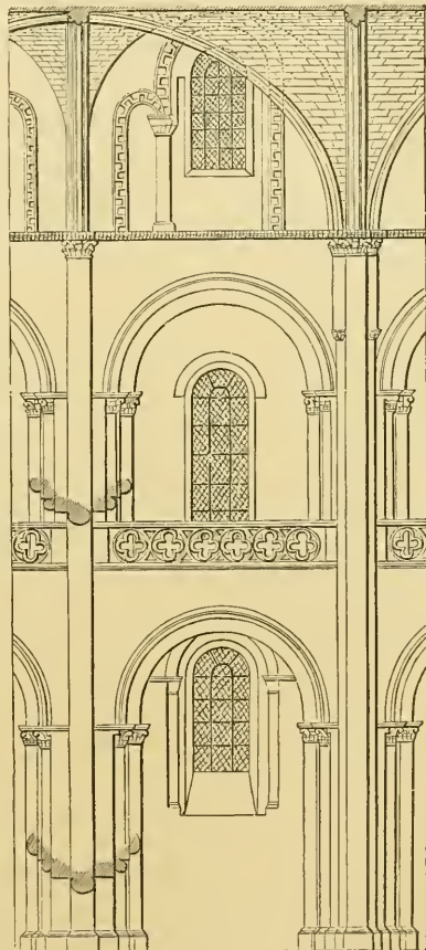
616. Elevation of Compartment of Nave of St. Stephen, Caen. (From Pugin.)
