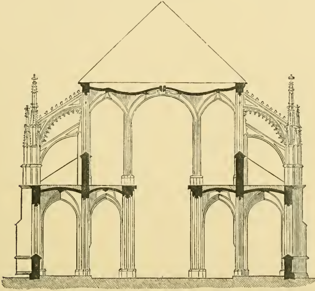
Section of the Church of St. Barbara, Kuttenberg. Scale 50 ft. to 1 in.
