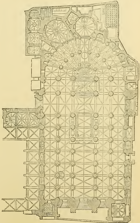
940. Plan of Cathedral at Toledo. (From 'Monumentos Arquitectonicos d'Espana.'). Scale 100 ft. to 1 in.
