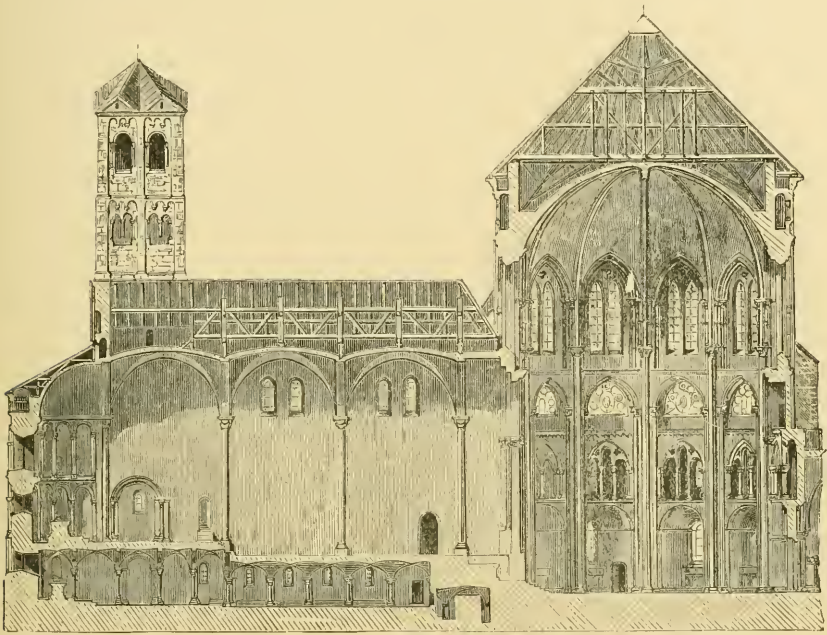
740. Section of St. Gereon, Cologne. (From Boisserée, 'Nieder Rhein.')
