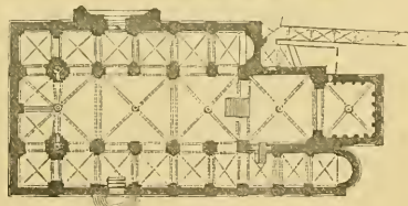
722. View and Plan of the Cathedral at Zurich. (From Voselin.) Scale 100 ft. to 1 in.
