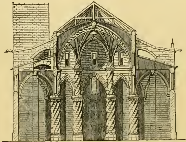
956. Section of Church at Villena. (From 'Mon. Arch. d'España.')
