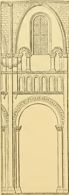
617. Compartment, Abbaye-aux-Dames, Caen. (From Pugin.)
