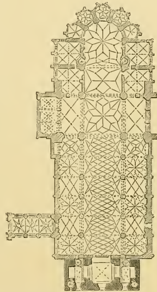
681. Plan of St. Jacques, Liège. (From Weale's 'Architectural Papers.') Scale 100 ft. to 1 in.
