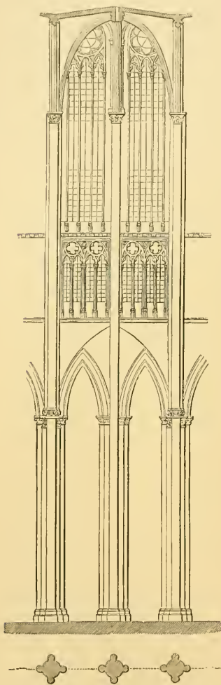
630. Bay of Nave of Beauvais Cathedral. No scale.
