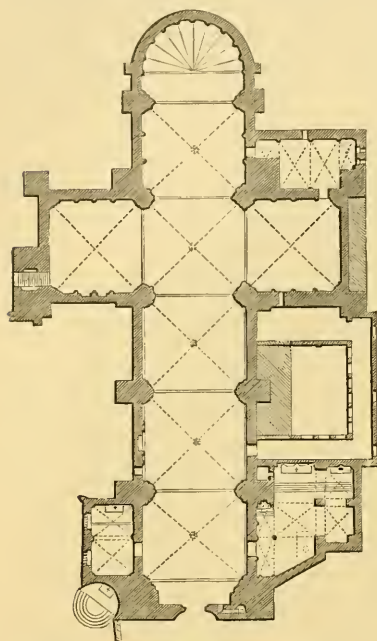
583. Cathedral at Angers. (From Fau'trier, Anjou et ses Monuments. ) Scale 100 ft. to 1 in.
