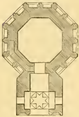
1001. Plan of Tomb of Zobeidé, Bagdad. Scale 100 ft. to 1 in.
