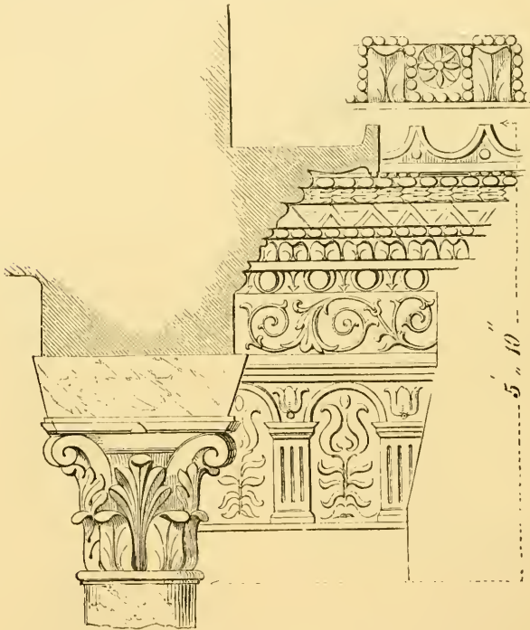
Order of the Dome of the Rock. (From a Drawing by Arundale.)
