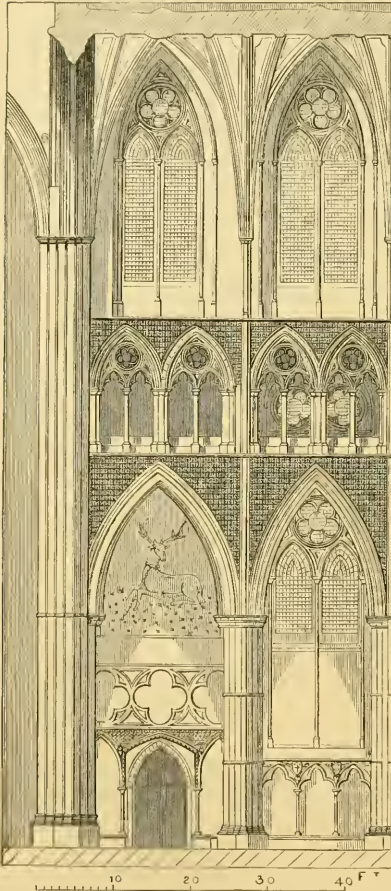
822. Two Bays of the Nave of Westminster Abbey. Scale 25 ft. to 1 in.
