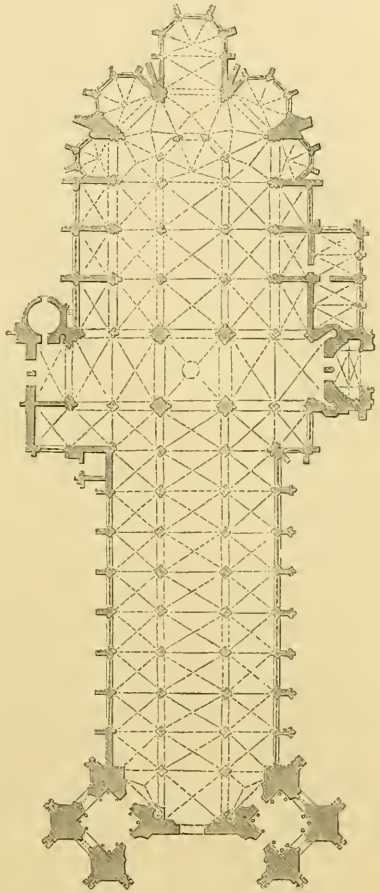
645. Plan of Church of St. Ouen at Rouen. (From Peyrée's 'Manuel.') Scale 100 ft. to 1 in.
