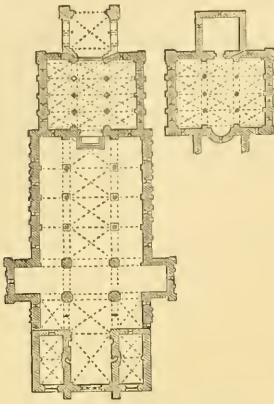
689. Plan of the Church at Romain-Motier. (From Blavignac. 2 ) Scale 100 ft. to 1 in.
