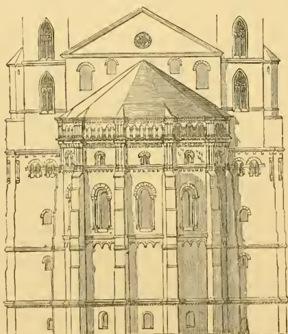
698. Eastern Apse of Church at Trèves. (From Schmidt.) Scale 50 ft. to 1 in.
