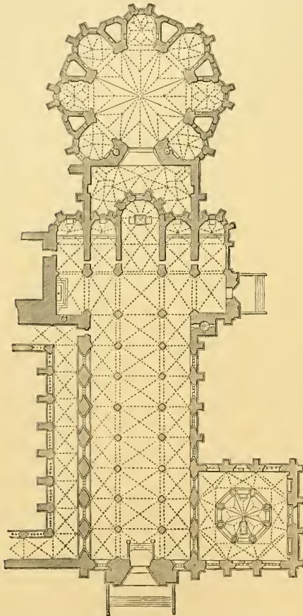
968. Plan of the Church at Batalha. (From Murphy.) Scale 100 ft. to 1 in.
