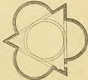
556. Plan of Church at Planes. (From Taylor and Nodier.)
