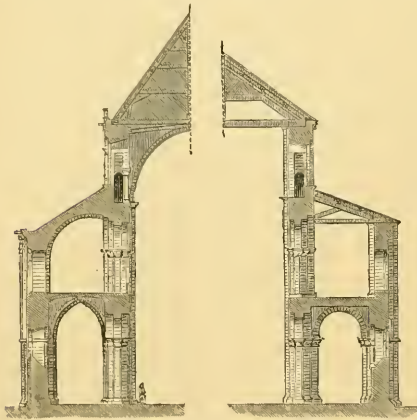
614. Fig. 1, after Vaulting; Fig. 2, before Vaulting. Section of Nave of St. Stephen, Caen.
