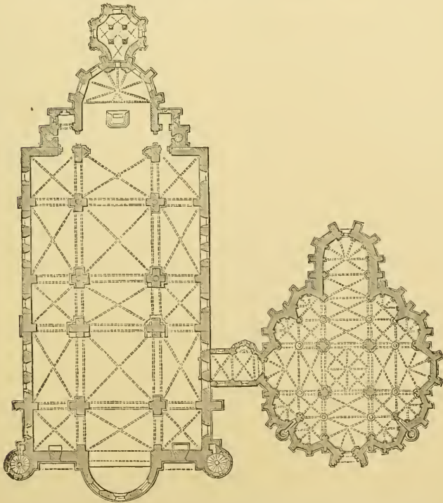
696. Plan of Medieval Church at Trèves. (From Schmidt, 'Baudenkmale von Trier.') Scale 100 ft. to 1 in.
