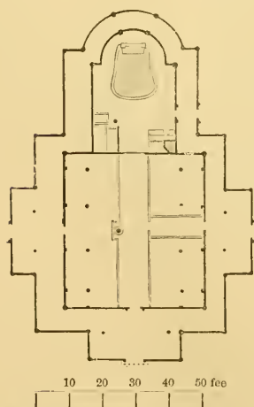
796. Plan of Church at Hitterdal.
