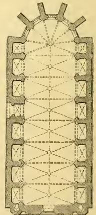
949. Sta. Maria del Pi, Barcelona. (From Street.) Scale 100 ft. to 1 in.
