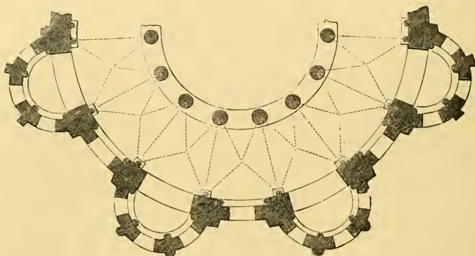
596. Plan of Chevet, Notre Dame du Port, Clermont. (From Chapuy.) No scale.
