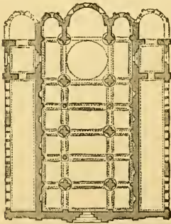
937. St. Millan, Segovia. (From Gaillhabaud.) Scale 100 ft. to 1 in.
