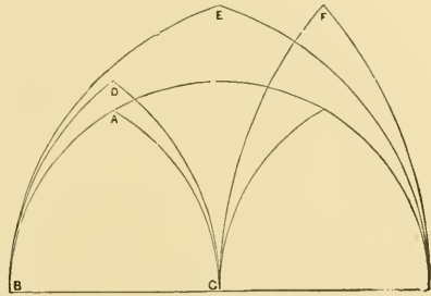
615. Diagram of Vaulting.
