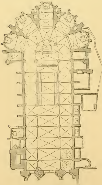
639. Plan of Cathedral at Bazas. (From Lamothe. 1 ) Scale 100 ft. to 1 in.
