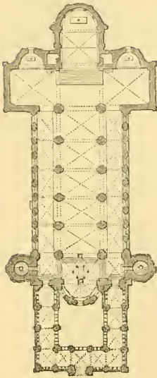
711. Plan of Church at Laach. (From Geier and Görz.)
