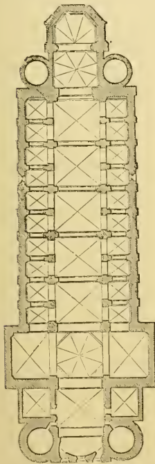
701. Plan of Cathedral of Worms. (From Geier and Görz.) Scale 100 ft. to 1 in.
