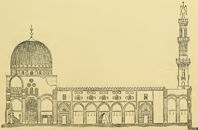
984. Section of Mosque of Berkook. (From Coste's 'Architecture Arabe.')
