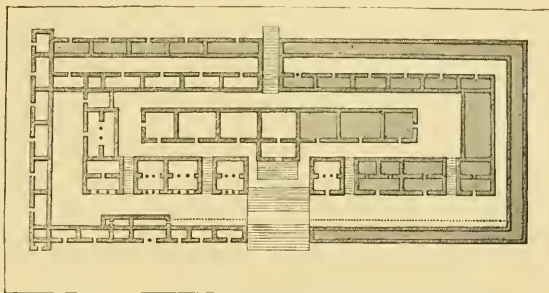
1022. Plan of Palace at Zayi. Scale 100 ft. to 1 in.
