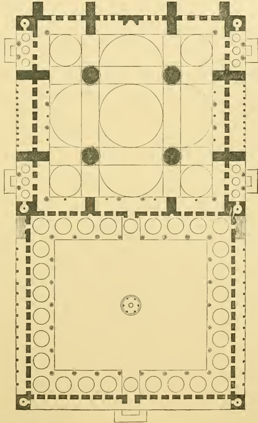
1000. Plan of Ahmedjic Mosque. (By Texier.) Scale 100 ft. to 1 in.
