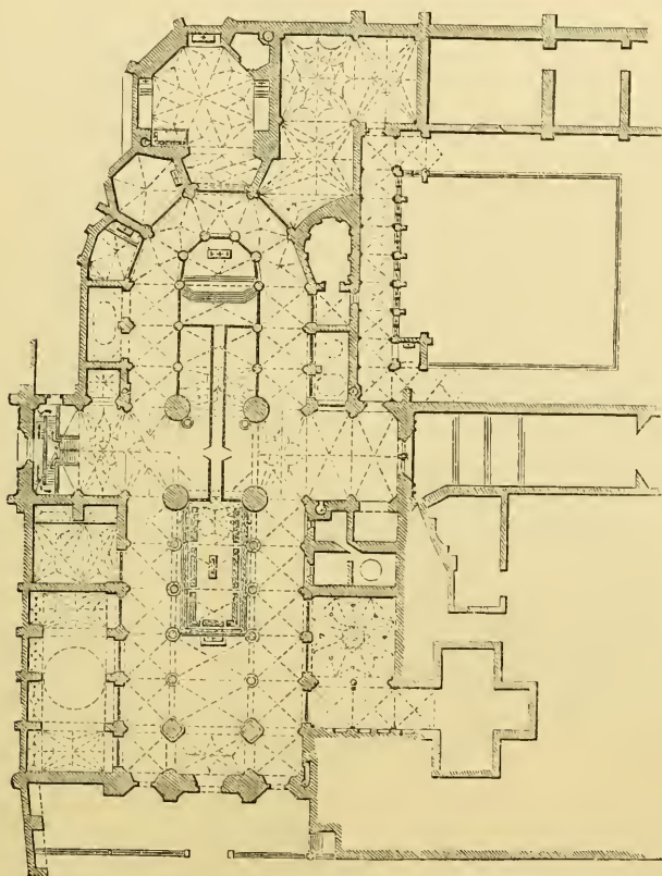
942. Plan of Burgos Cathedral. (Reduced from Street's.) Scale 100 ft. to 1 in.
