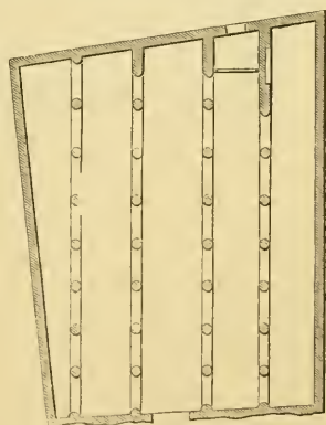
557. Sta. Maria la Bianca. (From 'Mon. Arch.'). Scale 50 ft. to 1.
