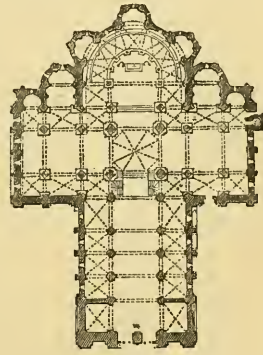
574. Plan of Church at Conques. (From Taylor and Nodier.) Scale 100 ft. to 1 in.
