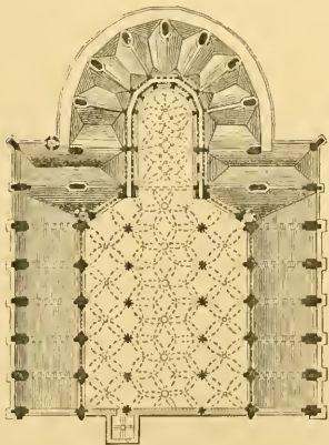
755. Plan of the Church at Kuttenberg, taken above the roof of the aisles. Scale 100 ft. to 1 in.
