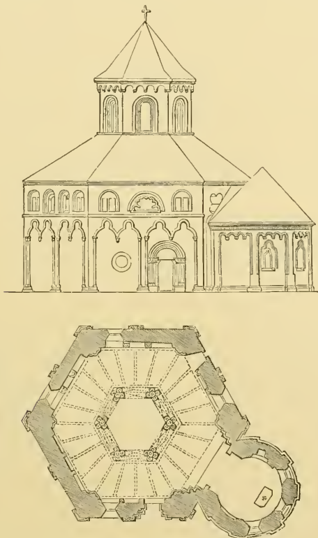
730. The Matthias Chapel at Cobern on the Moselle. (From Wiebeking.) No scale.
