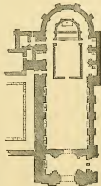
567. Plan of Church at Moissac. (From Taylor and Nodier.) Scale 100 ft. to 1 in.
