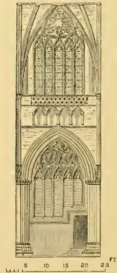
823. One Bay of Cathedral at Exeter. Scale 25 ft. to 1 in.
