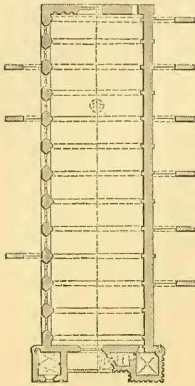
866. Plan of Westminster Hall. Scale 100 ft. to 1 in.
