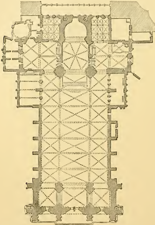
749. Plan of Strasburg Cathedral. Scale 100 ft. to 1 in.
