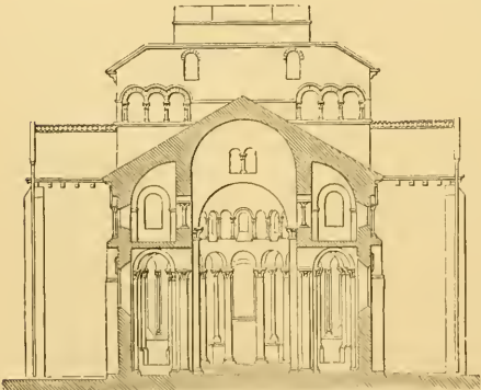
594. Section of Church at Issoire, looking East. (From Mallay.) Scale 50 ft. to 1 in.
