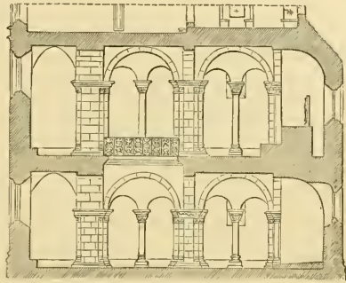
721. Section of Chapel at Landsberg. (From Puttrich.)
