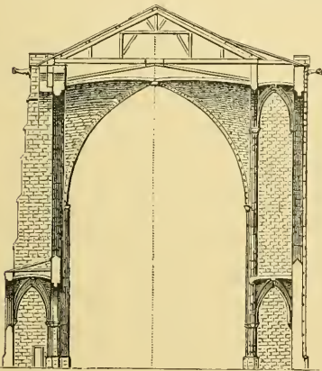
570. Section of Church of the Cordeliers at Toulouse. 50 ft. to 1 in. (From King's 'Study Book.')
