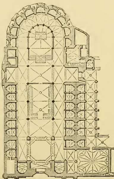
947. Plan of Cathedral at Barcelona. (Reduced from Street's.) Scale 100 ft. to 1 in.
